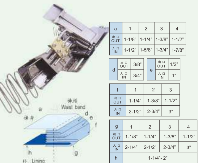
JZ-15540 F324 西裤裤头贴拉筒 Casual Trousers Waist Band Folder
