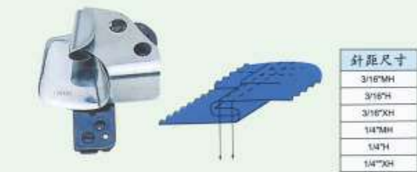
JZ-15525 35800(F337) 弹弓嘴迂仁埋夹 Sprig Type Side Seam Folder-Union Special Type
