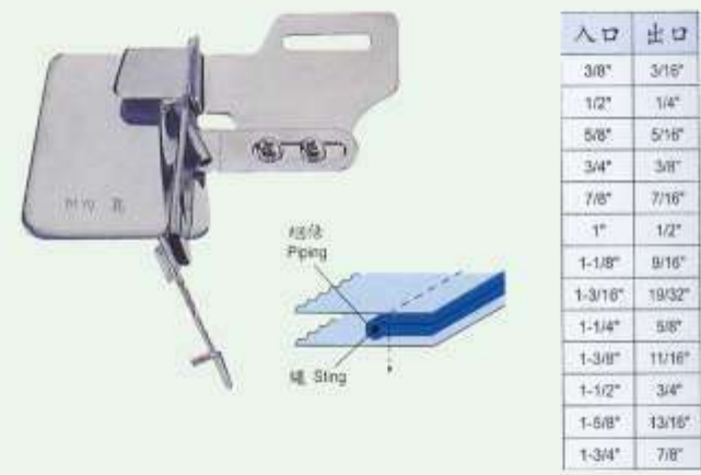
JZ-15534 432 绳子筒(固定式) Piping Folder
