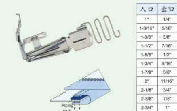
JZ-15527 F400 绷缝车直角包边筒(插凹子母筒单折可调) Right Angle Binder with Piping
