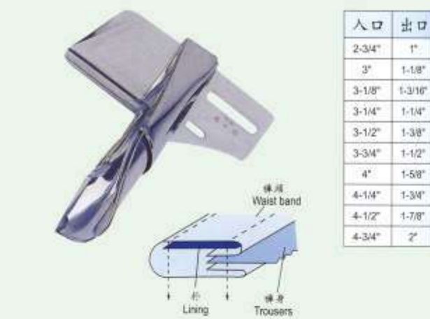
JZ-15529 F302 裤头筒有补 Waist Band Folder With Lining
