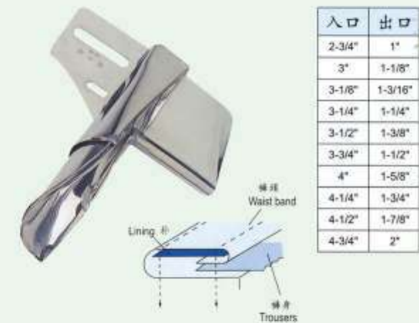
JZ-15530 F304 散底裤头筒有补 Waist Band Folder With Lining
