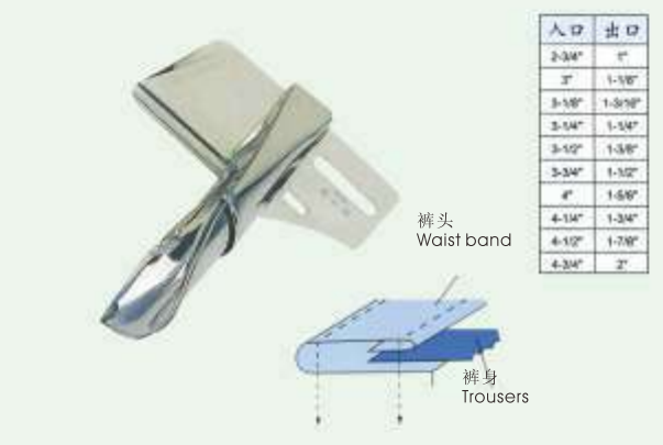
JZ-15521（F303）散底裤头筒 Waist Band Folder
