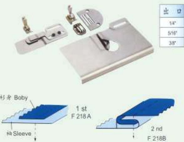
JZ-15533 F218 单针接袖器(单针车用) Single Needle Sleeve Attachment (Single Needle Operation)
