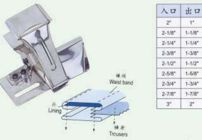
JZ-15537 F307 上下布裤头筒 Two Pieces Waist Band Folder
