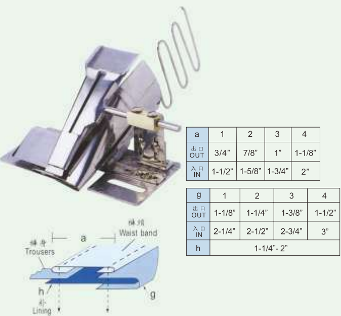
JZ-15541 F325 西裤裤头拉筒 Casual Trousers Waist Band Folder
