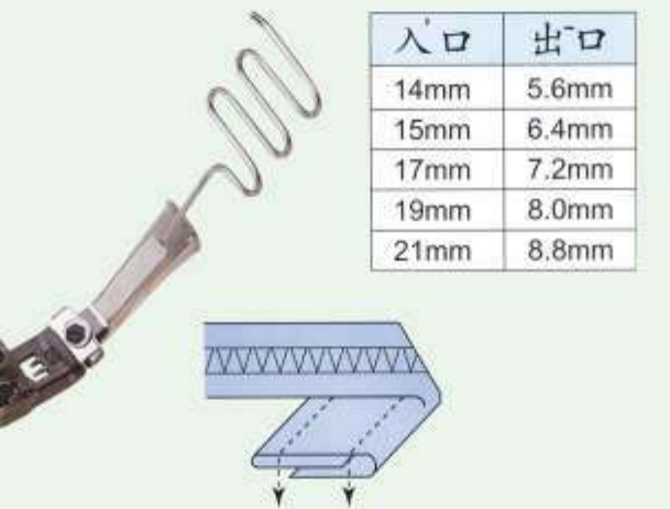
JZ-15539 443 绷缝车細条面贴器 Tape Attach Folder for Covering Stitch
