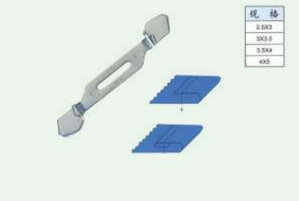
JZ-15522 U12 雨伞筒 Twin Plain Hemmer
