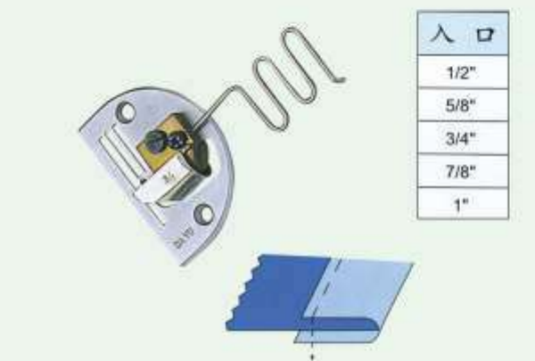
JZ-15518散口鞋边包边筒 Single Needle Binders(for Shoes)
